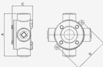
TAMPA PARAFUSADA
